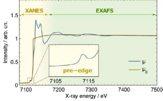
Figure 7: X-ray absorption spectrum of [\text{Fe}(\text{terpy})_2]^{2+} at the Fe K edge, showing the XANES and EXAFS regions together with the background contribution \mu_0 . The spectrum illustrates why the beam energy is chosen above the absorption edge, while avoiding the strongest near-edge structure [4].
