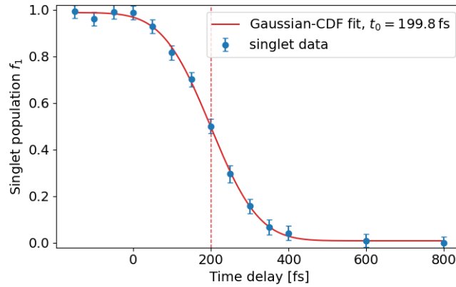
Figure 21: Singlet population extracted from the spectral decomposition together with the Gaussian temporal-transition fit. The fitted midpoint t_0 marks the effective temporal position of the excitation, while the fit width describes the finite temporal spread of the pump-probe response.
