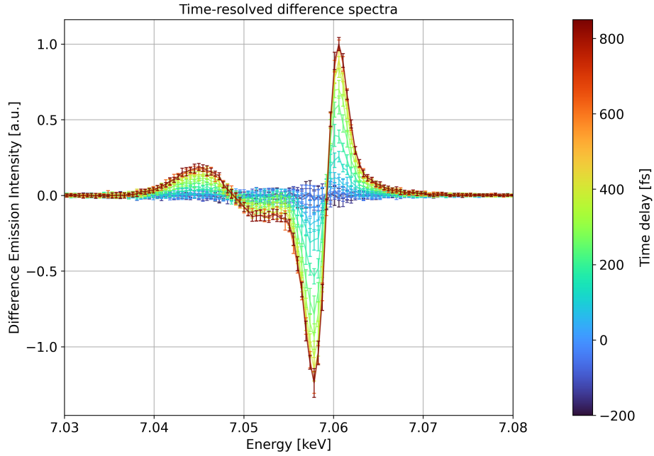
Figure 18: Transient X-ray emission spectra recorded at different pump-probe delays. Their evolving positive and negative features reveal the spectral changes associated with the population transfer between spin states.
