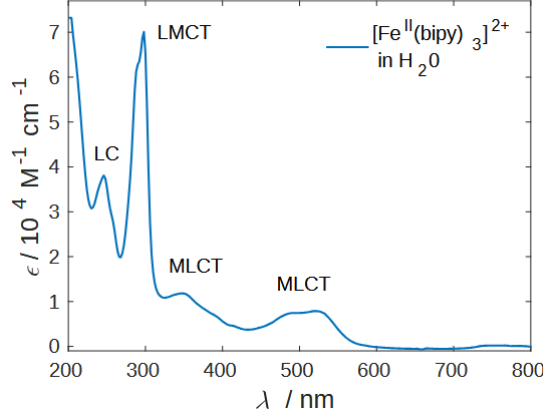
Figure 11: UV/VIS absorption spectrum of an aqueous [\text{Fe}(\text{bipy})_3]\text{Cl}_2 solution with the different charge-transfer transitions indicated. The wavelength-dependent absorption is used to estimate suitable concentrations and to compare the available excitation wavelengths [4].
