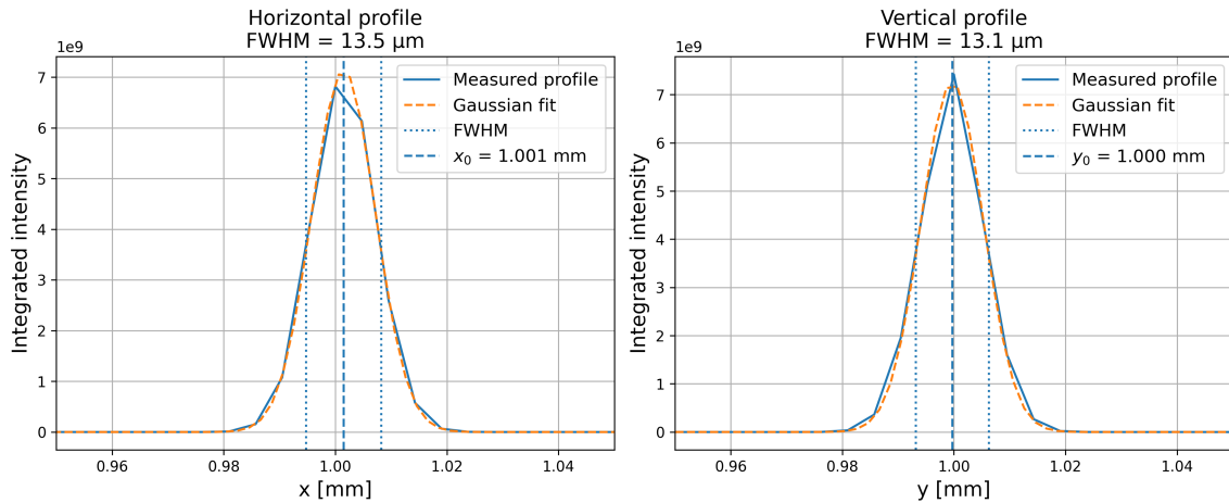
Figure 13: Spatial intensity profile of the focused X-ray beam in the sample plane. This measurement defines the probe-beam position and size at the liquid jet.
