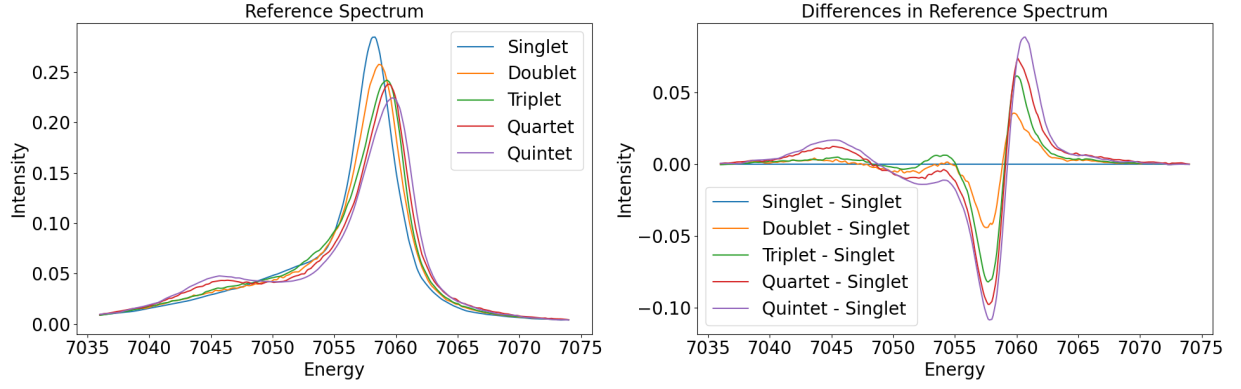
Figure 16: Reference X-ray emission spectra for the different spin states together with the corresponding reference difference spectra. These spectra provide the basis for identifying the spin-state contributions in the measured transient signal.
