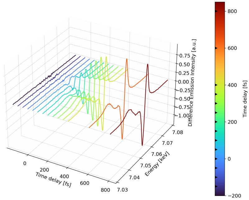
Figure 22: Three-dimensional representation of the time-resolved transient X-ray emission spectra. The additional view highlights how the spectral features evolve continuously with the pump-probe delay.
