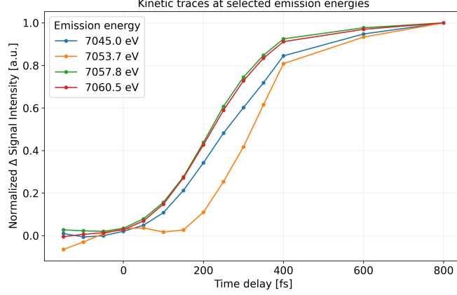
Figure 19: Kinetic traces of the transient signal at four selected emission energies as a function of pump-probe delay. Comparing these energies shows that the spectral features change systematically in time, confirming that the signal contains measurable dynamics rather than isolated statistical fluctuations and providing suitable traces for the subsequent analysis.
