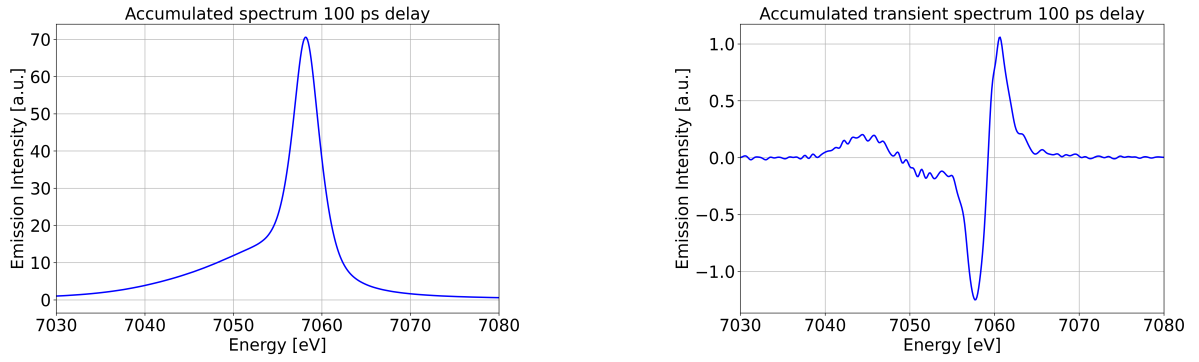
Figure 17: X-ray emission spectrum measured with the excitation laser on at a delay of 100 ps (left) and the corresponding laser-on minus laser-off difference spectrum (right). The comparison separates the dominant emission features from the transient changes caused by the optical excitation.
