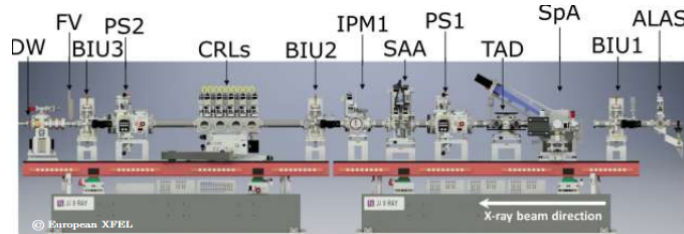
Figure 6: Overview of the FXE optical bench and its diagnostic and focusing components: BIU 1,2,3 (beam imaging units), SpA (spectrum analyser), TAD (time arrival detector), PS 1,2 (power slits), SAA (solid attenuator assembly), IPM1 (intensity position monitor), CRLs (compound refractive lenses) [4].
