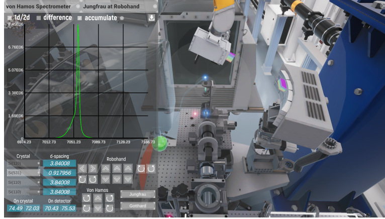
Figure 12: The Von Hamos spectrometer in its operating position, with the Jungfrau detector read-out shown alongside the instrument settings. This arrangement records the Fe K\beta emission spectrum over a broad energy range in a single measurement.
