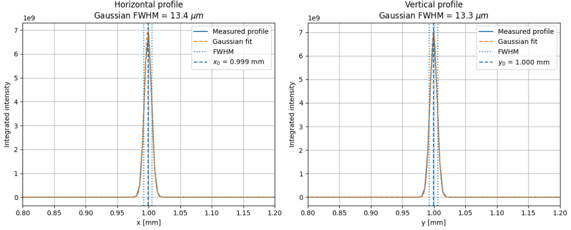
Figure 10: Horizontal and vertical intensity profiles of the focused X-ray beam together with Gaussian fits. The resulting FWHM of approximately 13.5 \mu\text{m} quantifies the beam size achieved at the focus.
