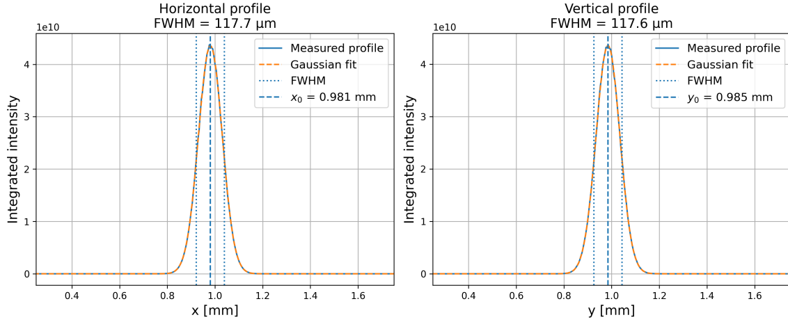
Figure 14: Spatial intensity profile of the optical excitation laser in the sample plane. Its broader profile is used to illuminate a larger region than the focused X-ray probe.
