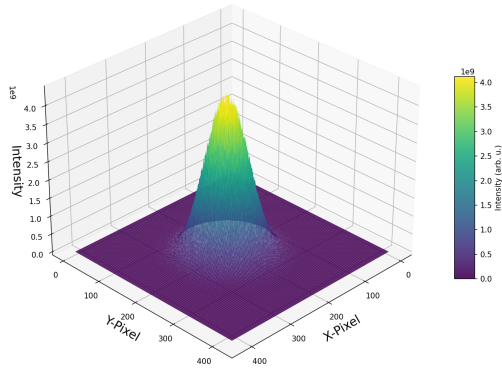
Figure 9: Three-dimensional intensity distributions of the pink beam (left) and the monochromatic beam (right) measured with identical attenuators. The plots show how the monochromator changes the recorded beam intensity while preserving the overall spatial beam profile.
