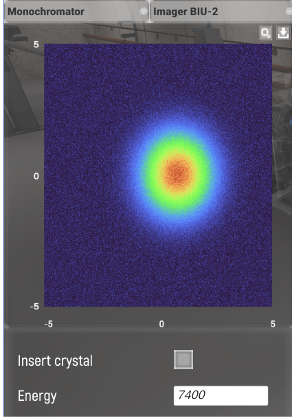
Figure 8: Beam images recorded with the same attenuator settings: the pink beam is shown on the left and the monochromatic beam on the right. The comparison makes the strong intensity loss caused by the monochromator visible, despite the improved spectral selectivity.
