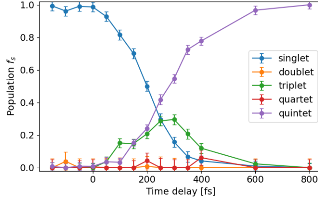
Figure 20: Fitted populations of the singlet, doublet, triplet, quartet and quintet reference states as a function of pump-probe delay. The transient triplet contribution and the subsequent growth of the quintet population support a relaxation pathway through an intermediate state.
